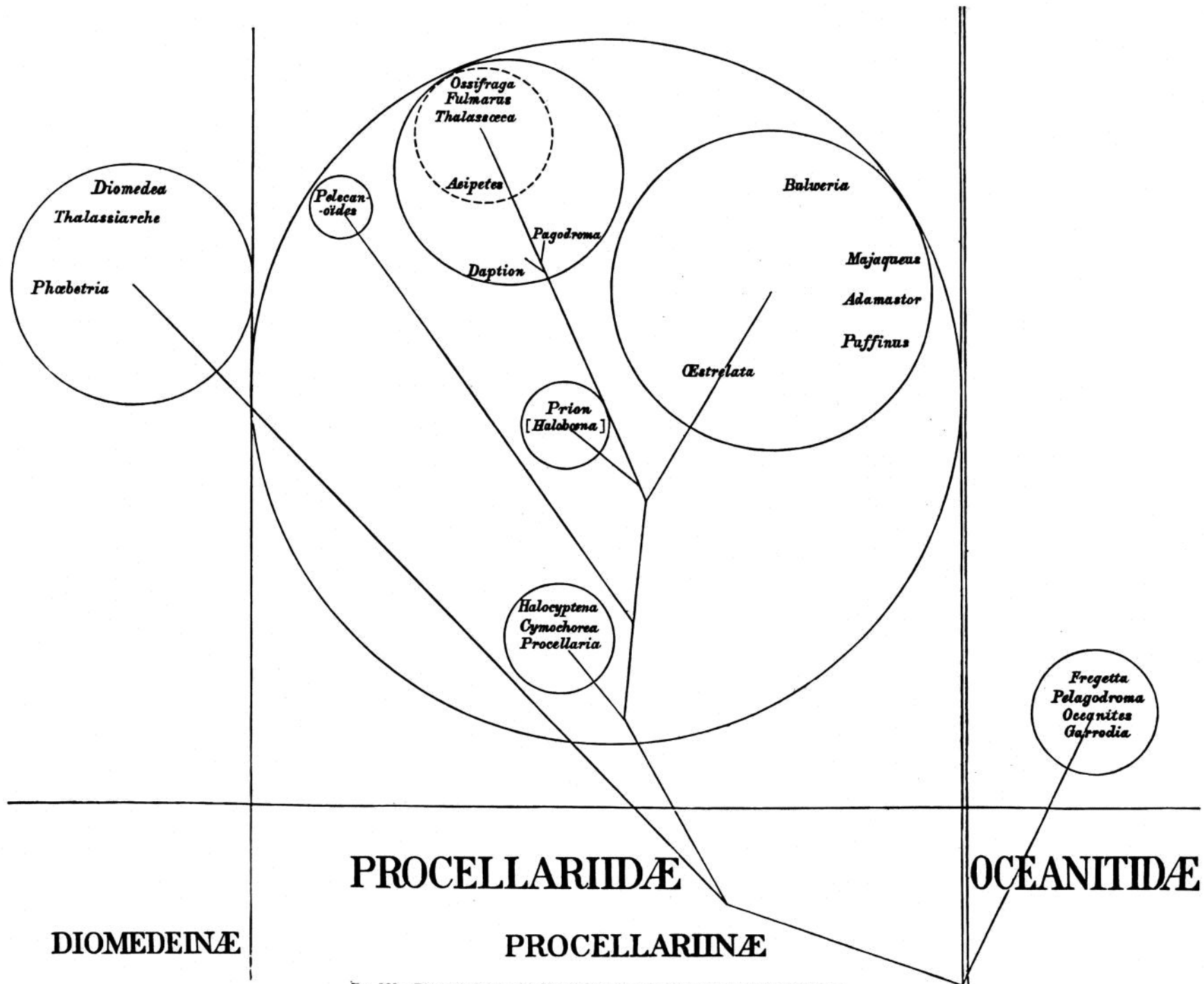
FIG. 132.—Diagram representing Mr. Forbes' view of the Classification of the Tubinares.
